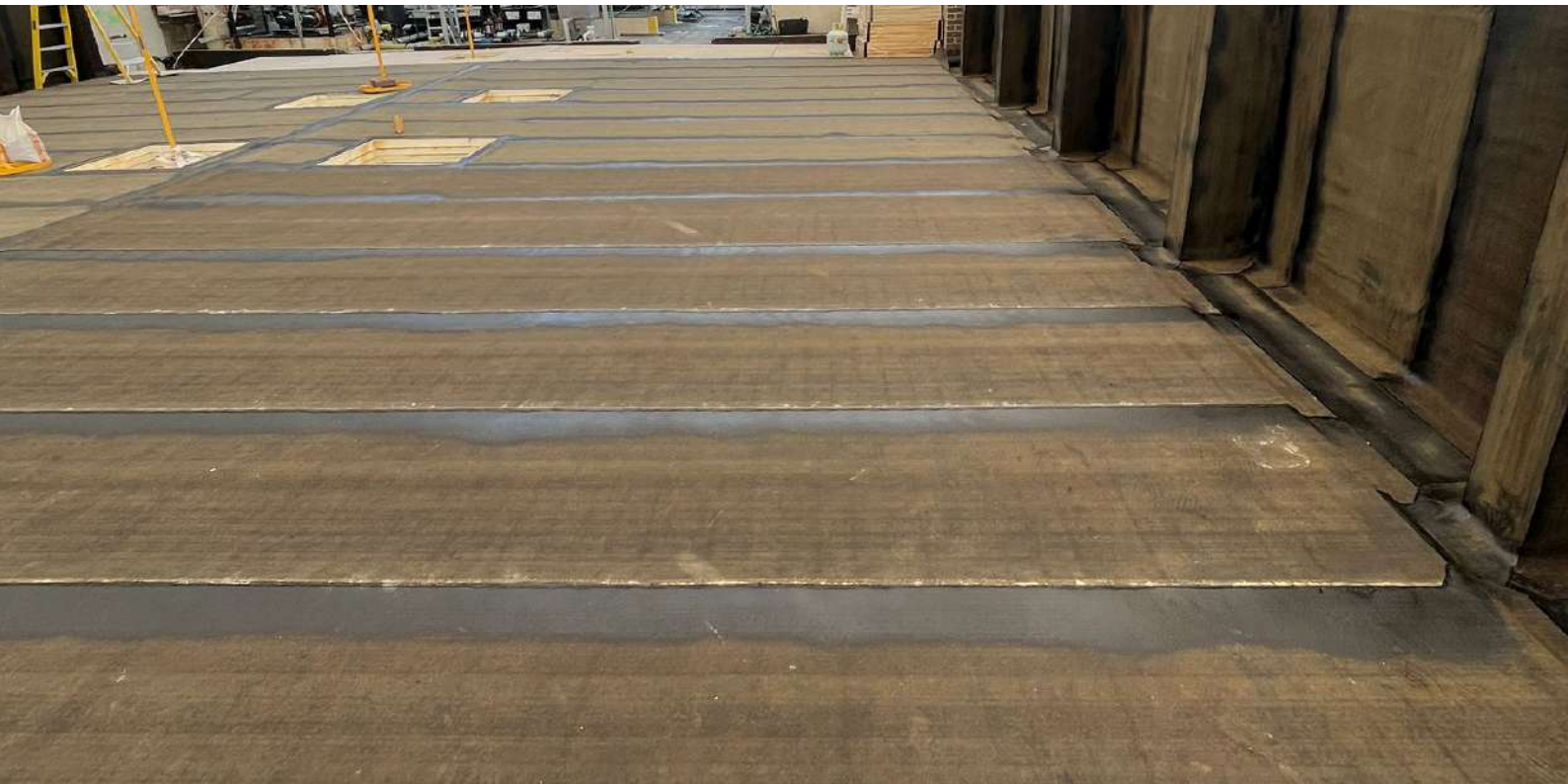
Second layer base sheet installed
