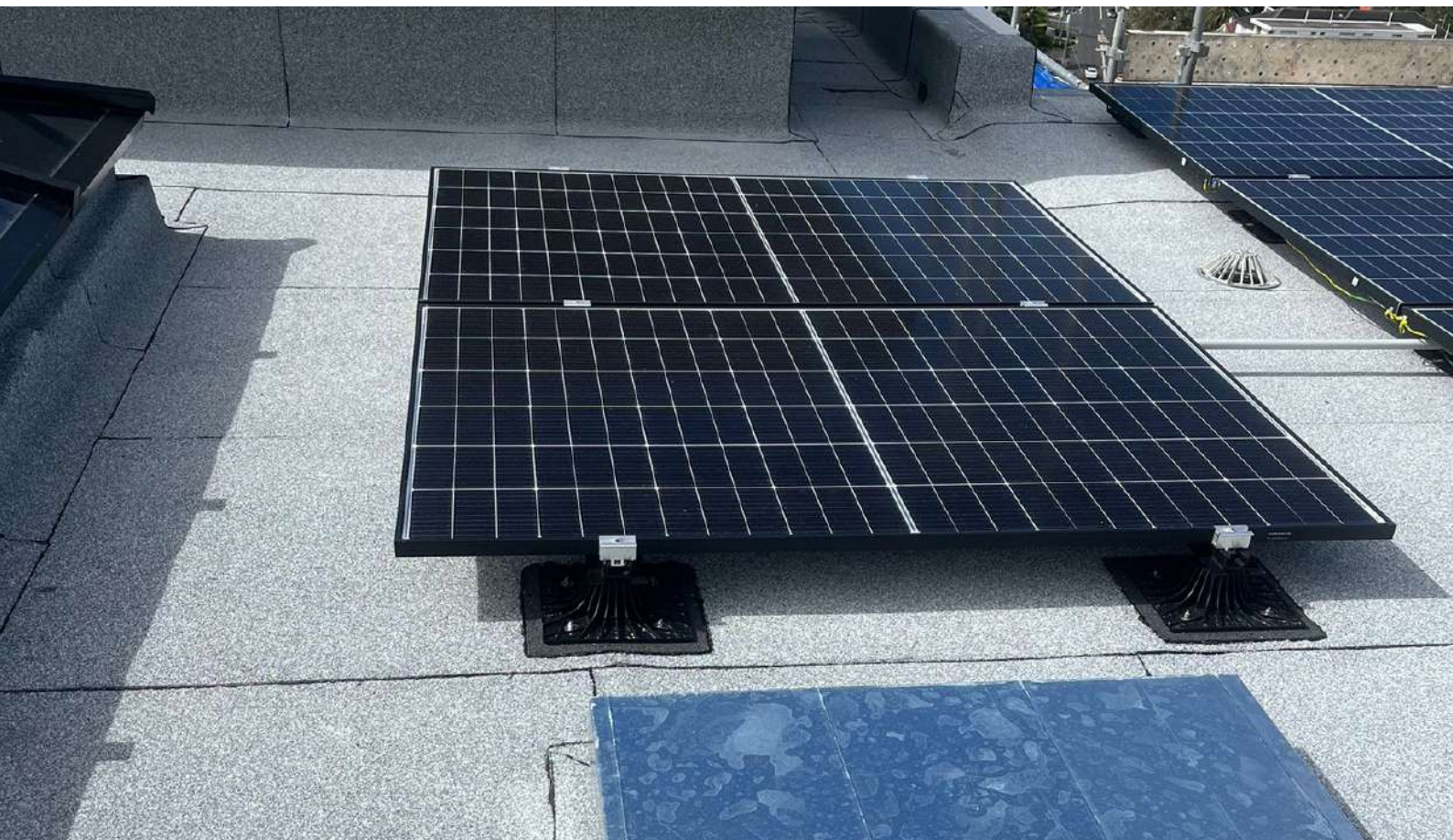
Panels installed on Enduroflex DuO Solar
