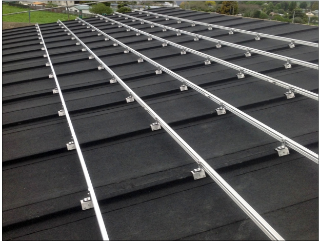
Framing ready for solar panels
