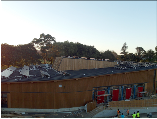
Main building completed roof - side view
