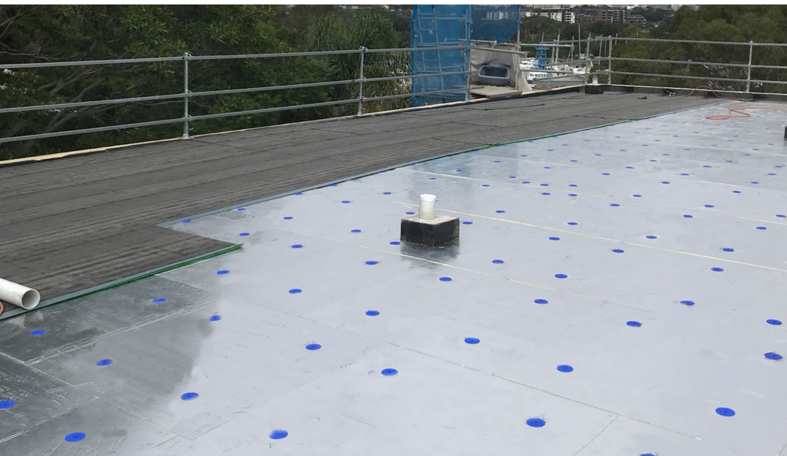
Basesheet installation
