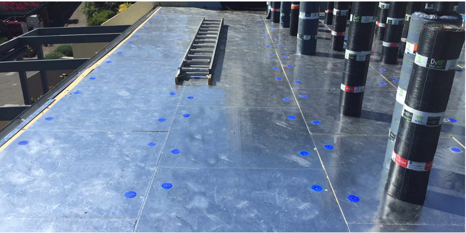
Insulation installation
