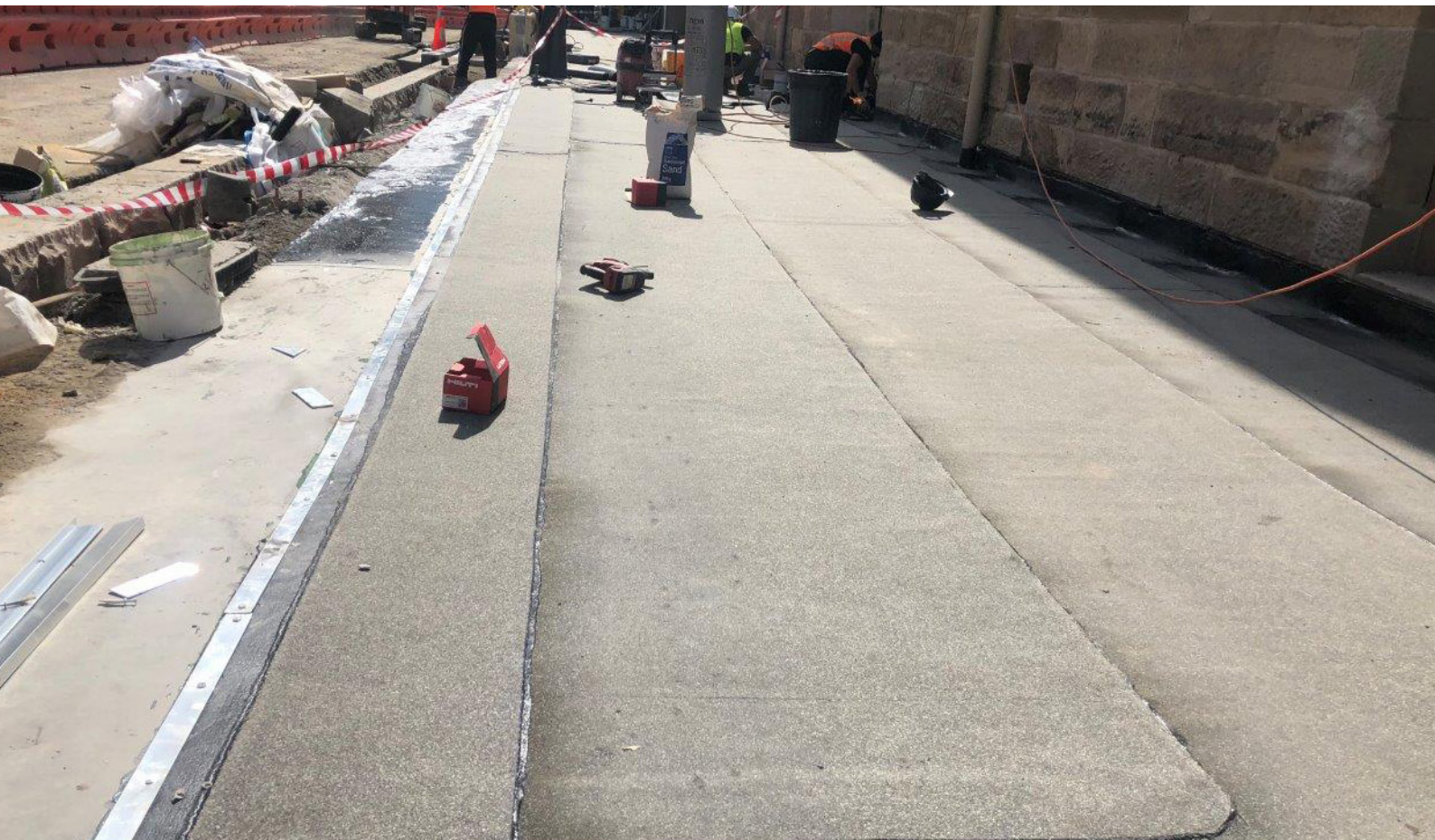
Installation of DuO B&T membranes
